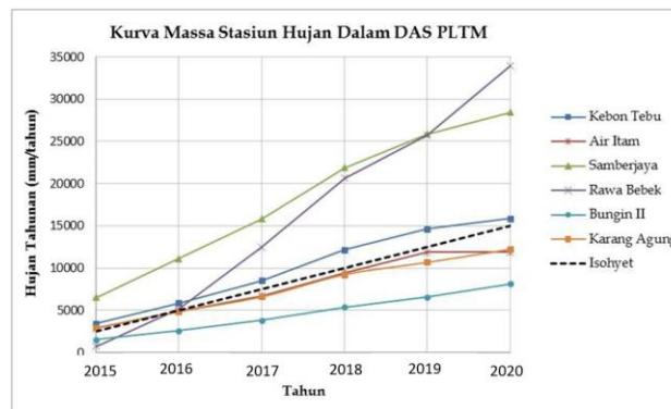
Figure 6. Mass Curve of All Rainfall Stations in the PLTM Watershed
